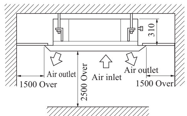
Installation space
